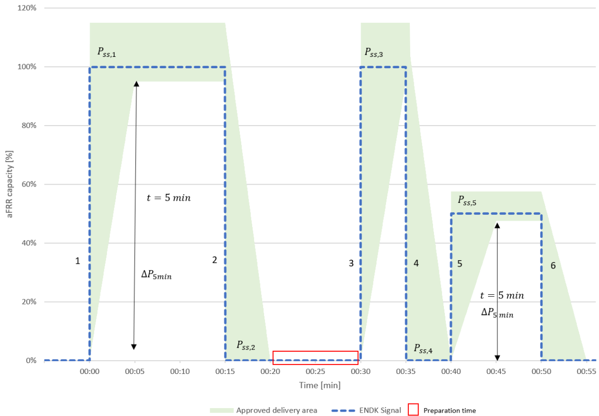
Figure 29 - aFRR functional test response for DK1 and DK2.
