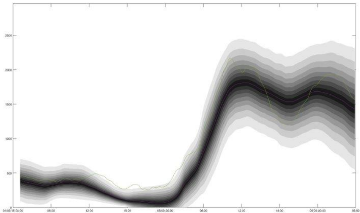
Figure 30 – Graphic illustration of application of 10% percentile in a probabilistic prognosis to estimate available capacity at the time of bidding for mFRR (9 o'clock, D-1).
