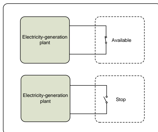
Figure 2 Possible exchange of external stop signal (available)
